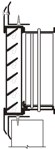
SSHFG/SSFG NO FC WITH OBD GRILLE MOUNTED
