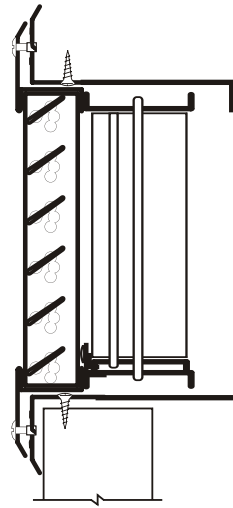
SSHFG/SSFG 1" OR 2" FC WITH OBD GRILLE MOUNTED
