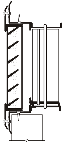
SSHFG/SSFG 1" FC WITH OBD MOUNTED TO PLASTER FRAME
