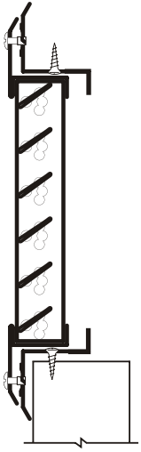
SSHFG/SSFG 1" FC BUILT INTO PLASTER FRAME NO OBD
