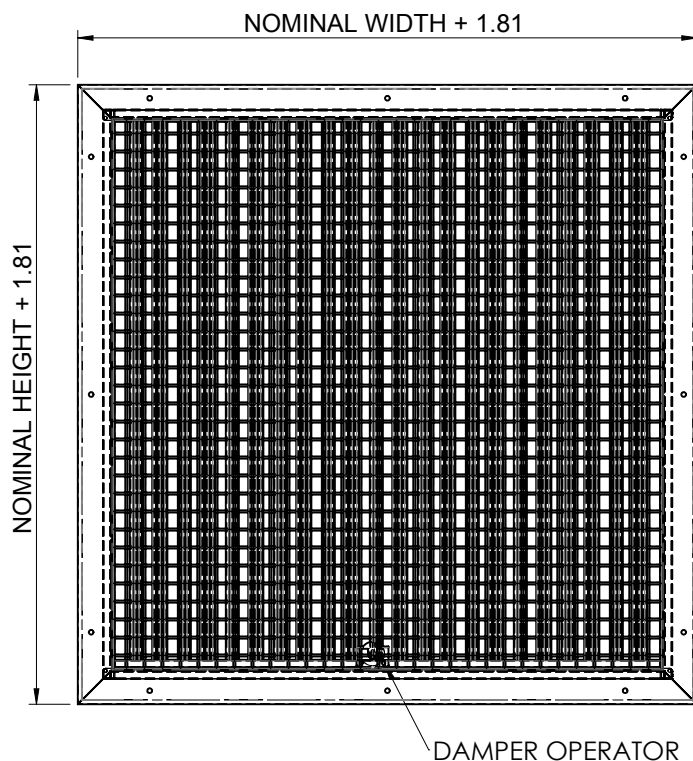
FACE VIEW
