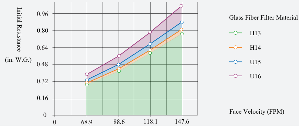
Chart of the Relationship Between Initial Resistance and Face Velocity
