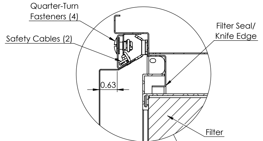
Filter Retainer Clips (No Tools Required)
