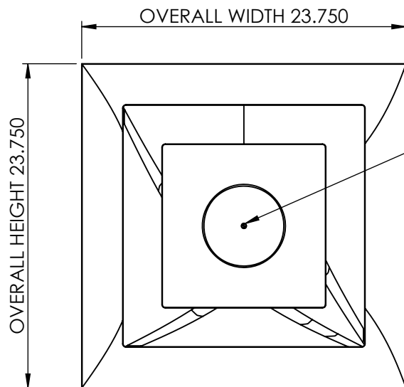
Removable Inner Cone Assembly
