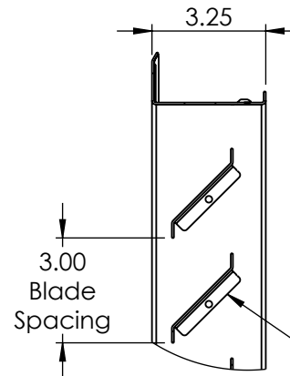
Example of 3" Blades
