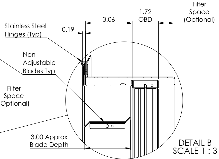
Example of 3" Blades @ 0°
