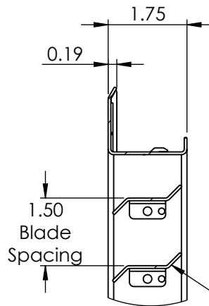
Example of 1.5" Blades @ 0°
