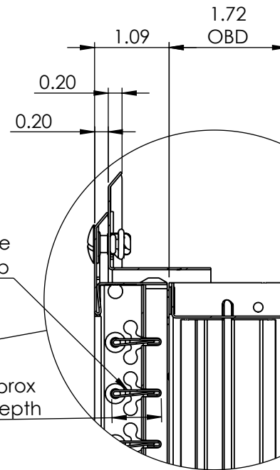
DETAIL B SCALE 1 : 2
