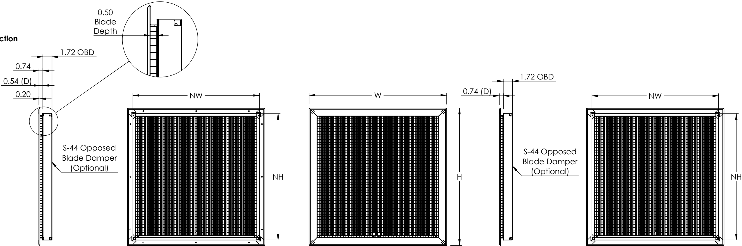
SURFACE MOUNT
