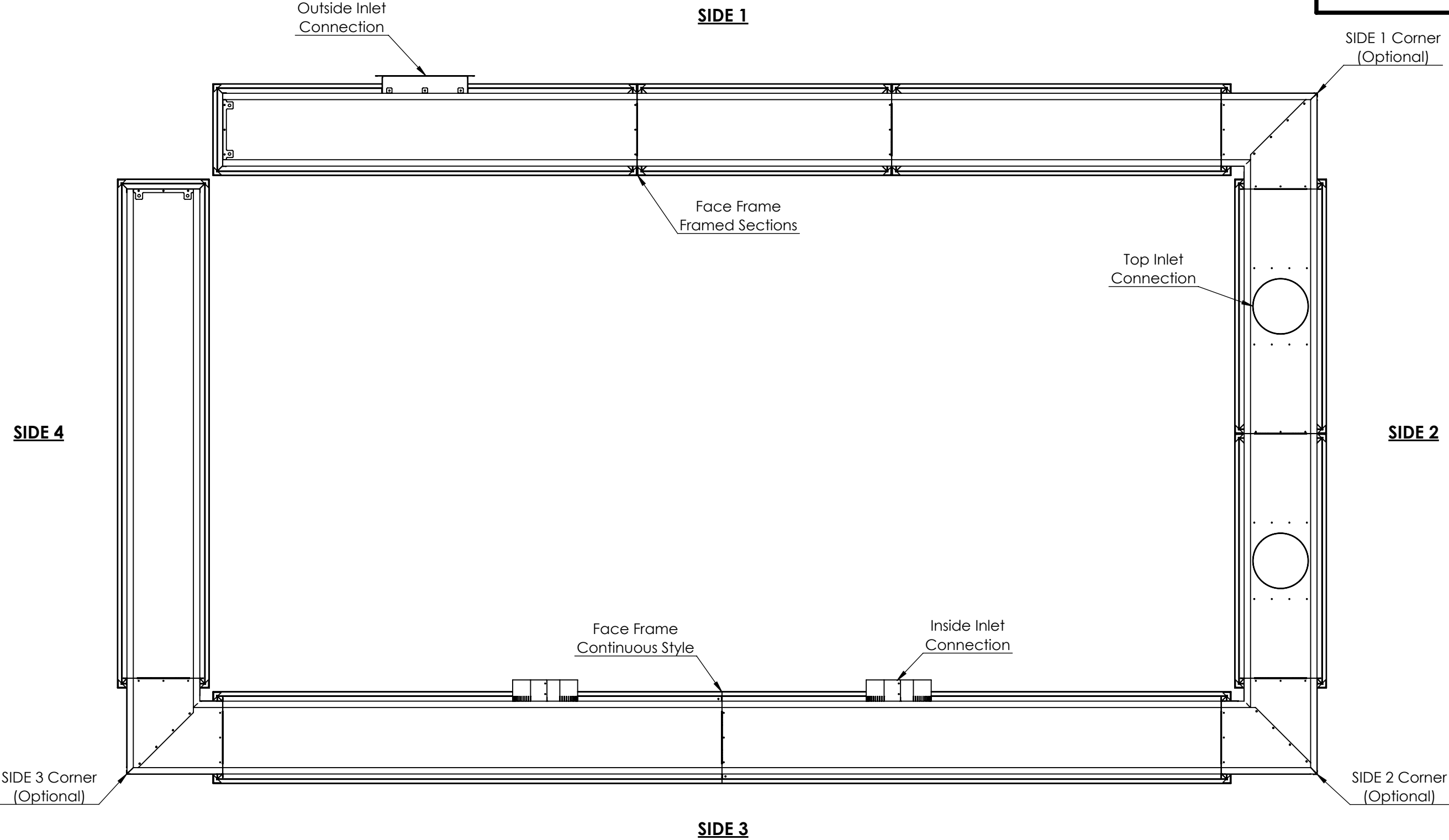
PLAN VIEW
