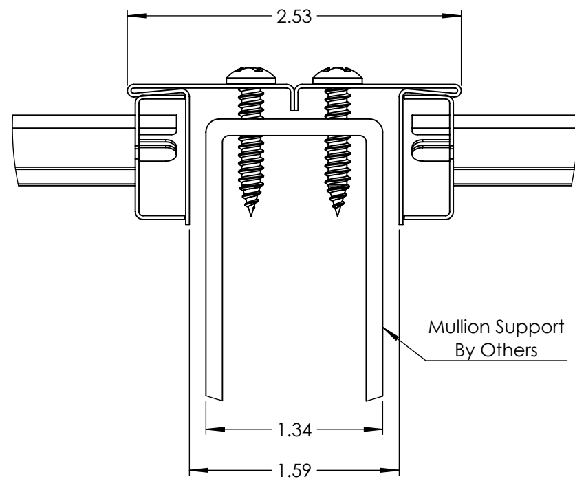
MULLION DETAIL ALL EXCEPT SSFG & SSHFG
