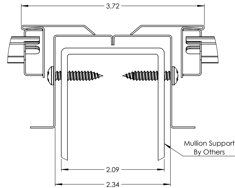
MULLION DETAIL SSFG AND SSHFG ONLY
