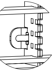
Concealed Mounting Tab Detail (Some Bars Removed for Clarity)
