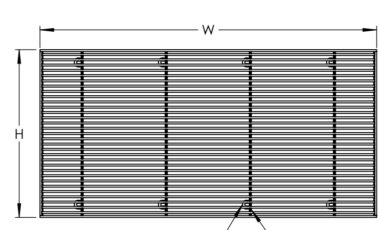
Concealed Mounting Tabs (Typ) Back Supports (Typ)
