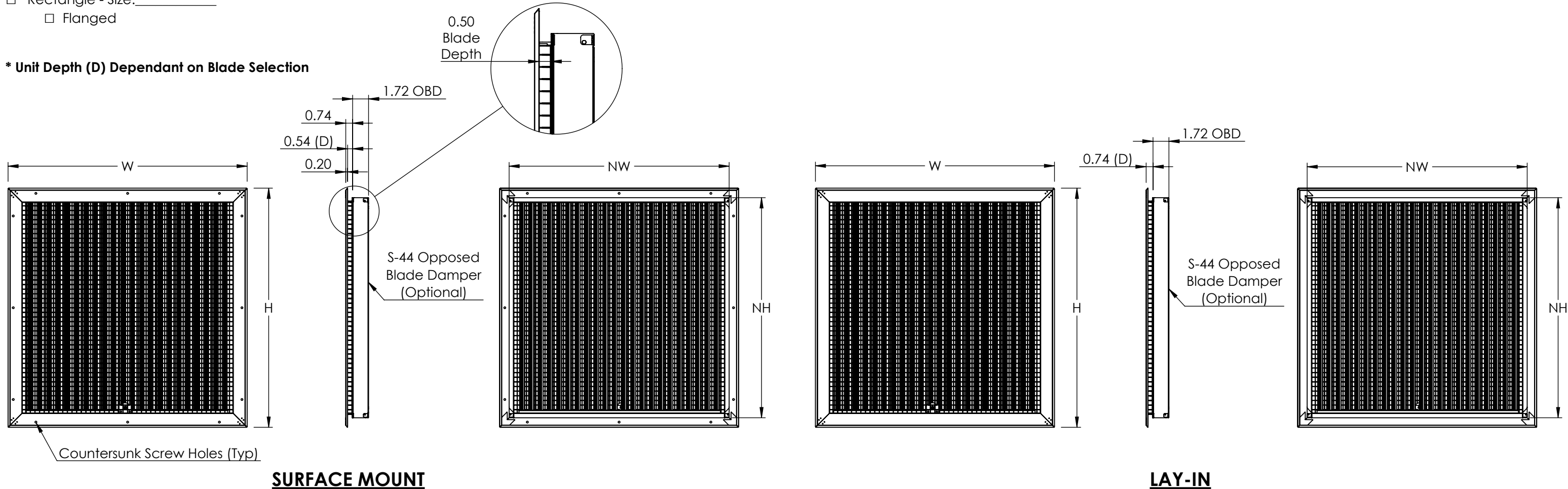
Lay-In
