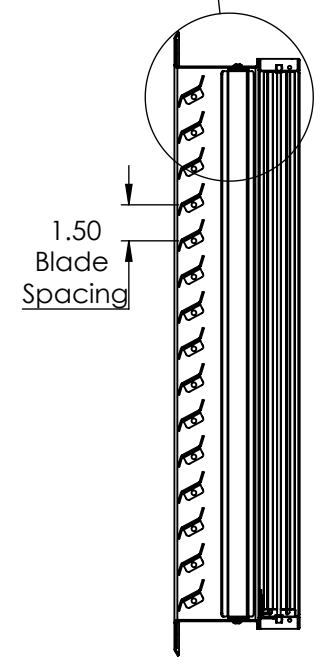
SURFACE MOUNT
