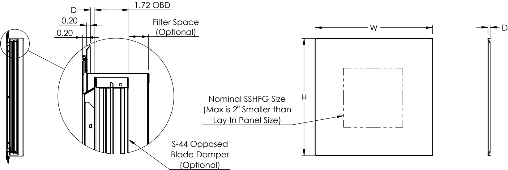
LAY-IN PANEL
