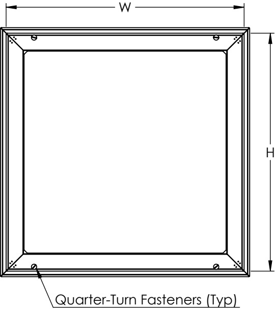
SURFACE MOUNT
