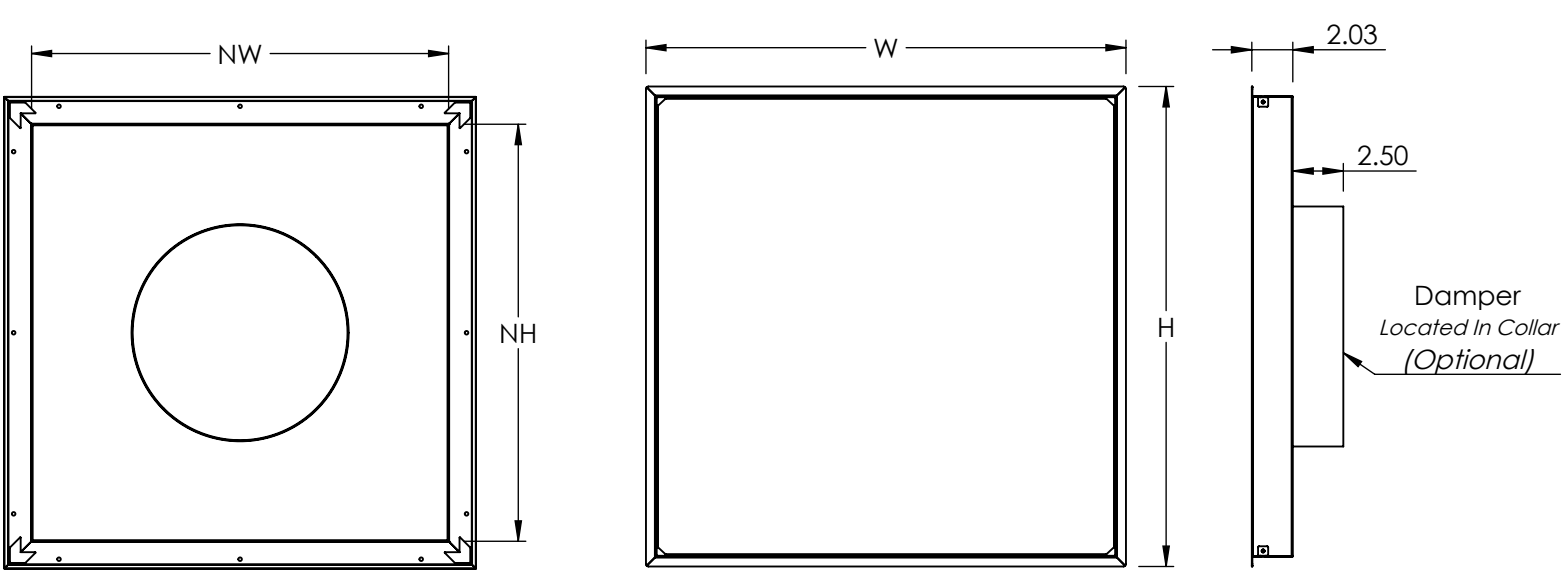
LAY-IN
