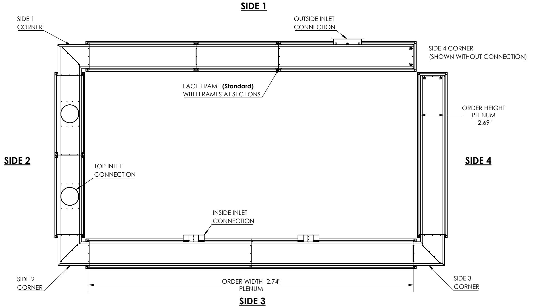
ROOM-SIDE VIEW
