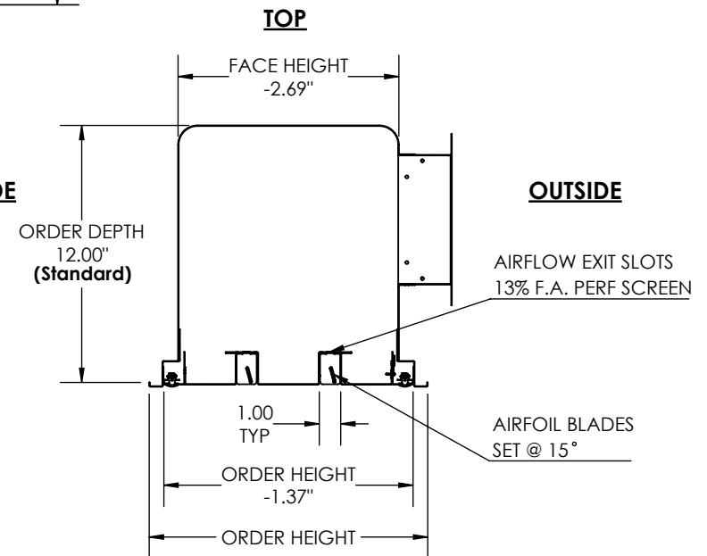
ROOM SIDE - CROSS SECTION
