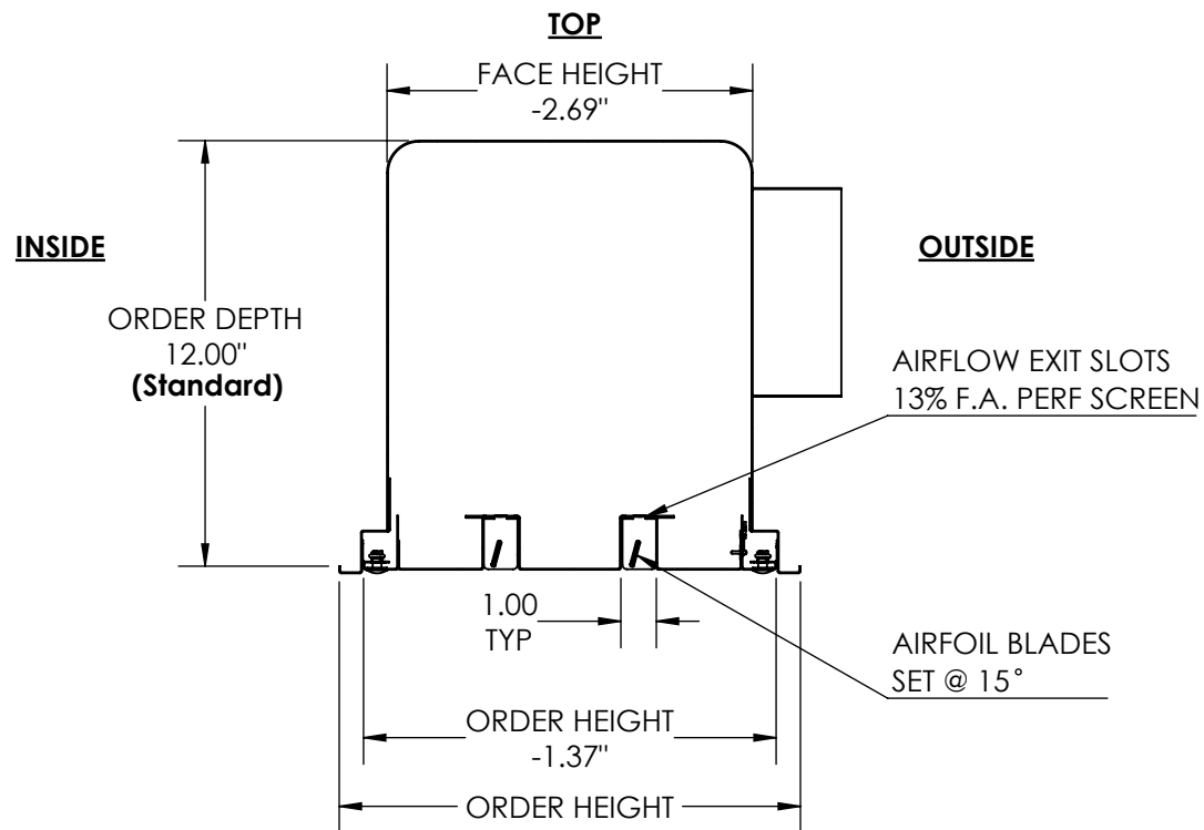
ROOM SIDE - CROSS SECTION
