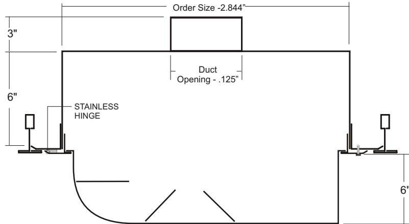
ONE-WAY BLOW
